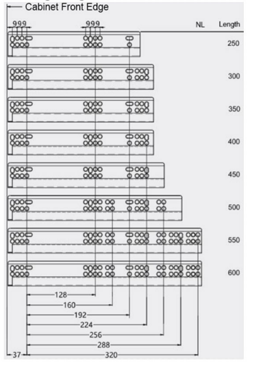
Drilling Diagram
