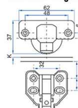
Installation Diagram
