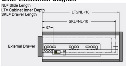
Slide Installation Diagram
