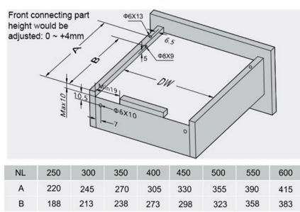
Drawer Installation Diagram
