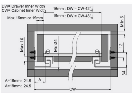
Slide Installation Diagram
