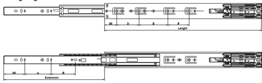
Drilling Diagram
