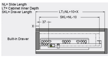
Drawer Installation Diagram
